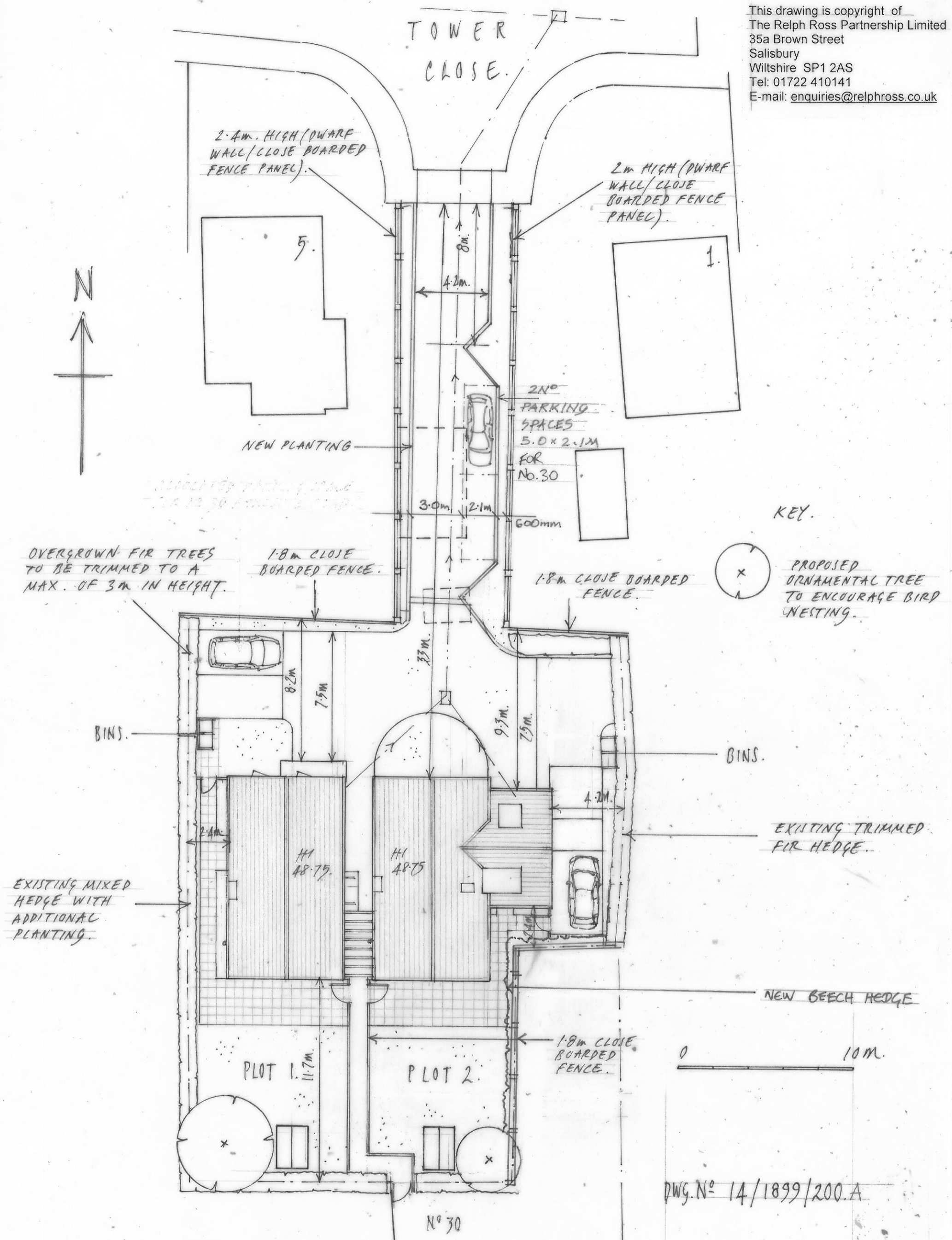
PROPOSED 2 x DWELLINGS ON LAND BETWEEN 1-5 TOWER CLOSE, CHARLTON, ANDOVER. SITE PLAN. SCALE 1:200 @ A3. JUNE '15.
